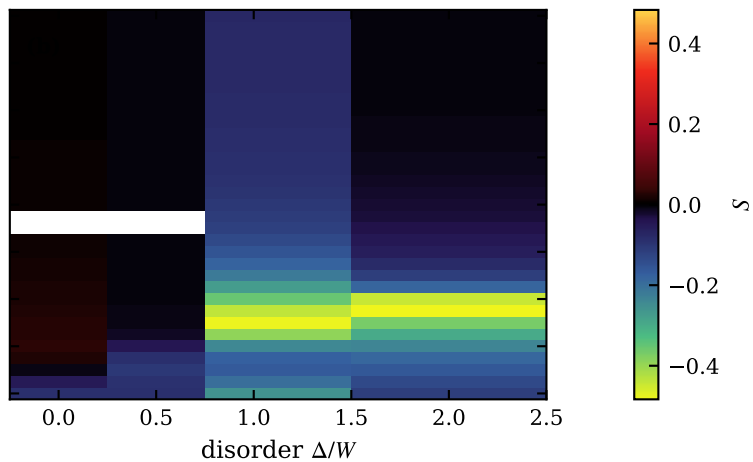
typ, n_c=0.24 , T/W=0.01 , \lambda=0
