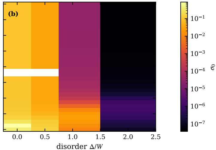
typ: \sigma(T \rightarrow 0) , n_c = 0.25 , \lambda = 0
