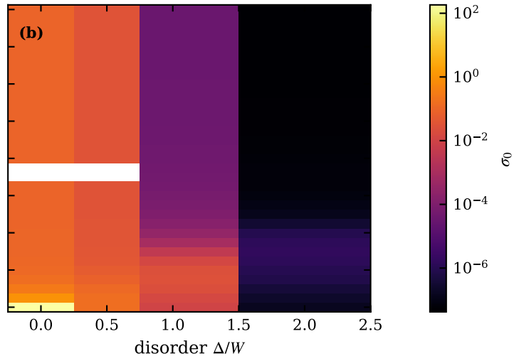
typ: \sigma(T \rightarrow 0) , n_c = 0.26 , \lambda = 0
