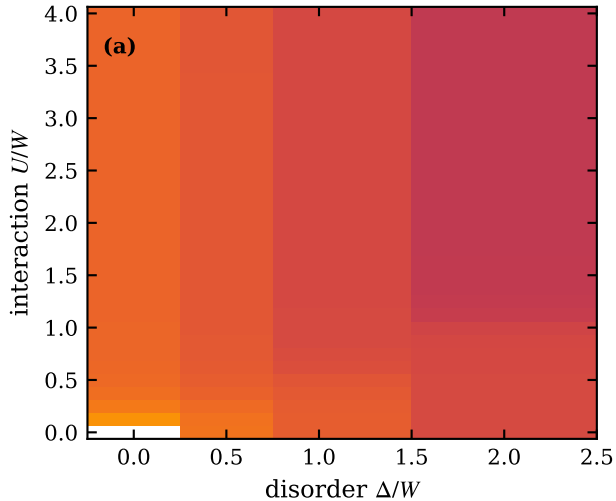
arith: \sigma(T \rightarrow 0) , n_c = 0.26 , \lambda = 0
