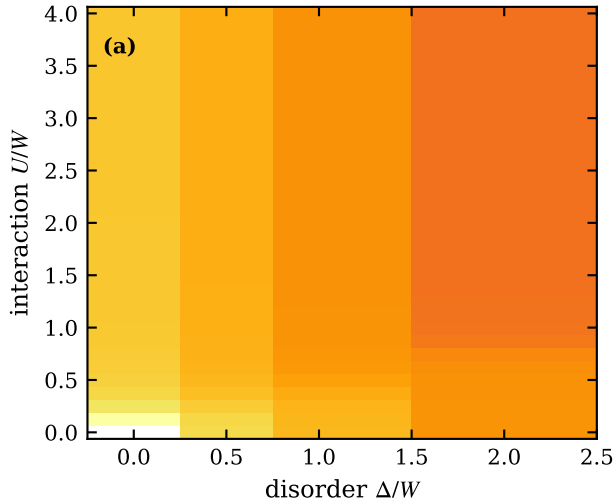
arith: \sigma(T \rightarrow 0) , n_c = 0.2 , \lambda = 0
