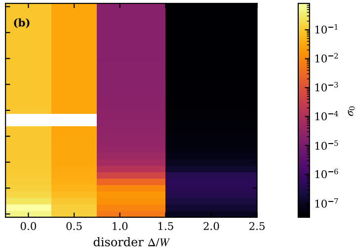
typ: \sigma(T \rightarrow 0) , n_c = 0.2 , \lambda = 0
