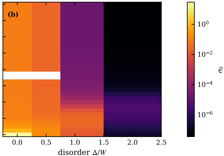
typ: \sigma(T \rightarrow 0) , n_c = 0.3 , \lambda = 0
