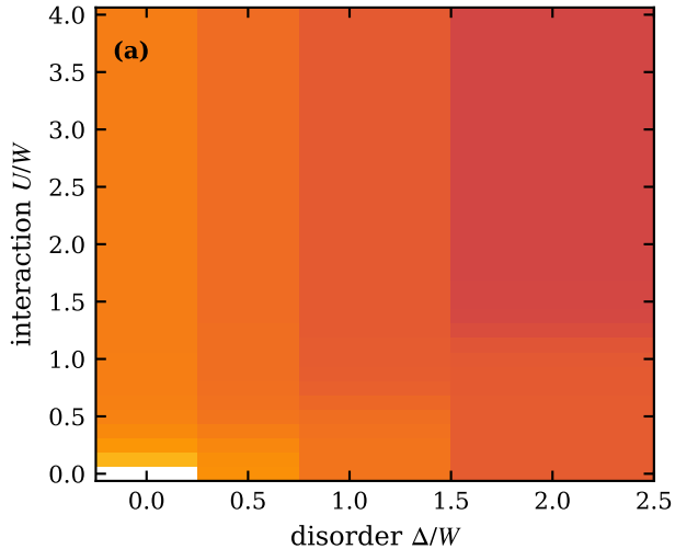
arith: \sigma(T \rightarrow 0) , n_c = 0.3 , \lambda = 0
