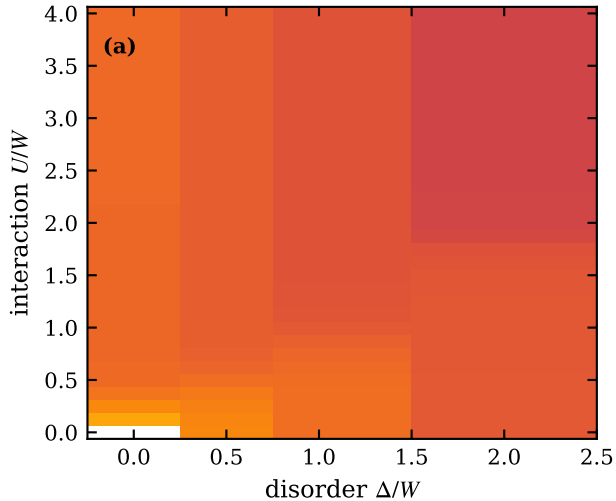
arith: \sigma(T \rightarrow 0) , n_c = 0.45 , \lambda = 0
