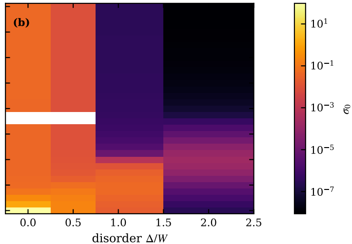
typ: \sigma(T \rightarrow 0) , n_c = 0.45 , \lambda = 0
