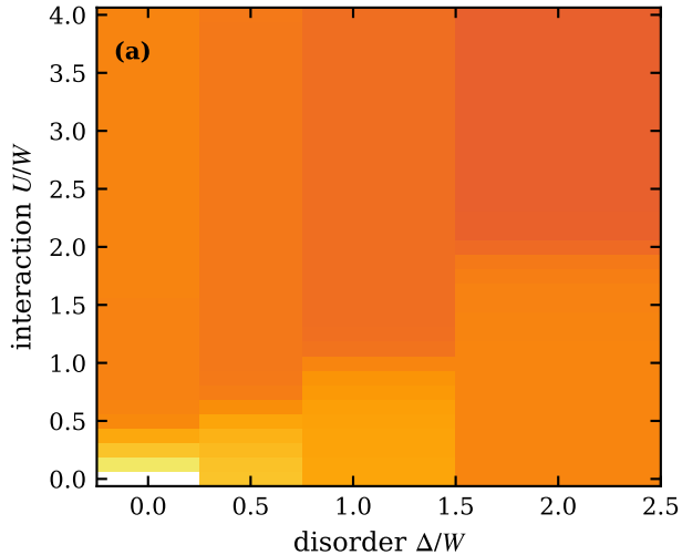
arith: \sigma(T \rightarrow 0) , n_c = 0.49 , \lambda = 0
