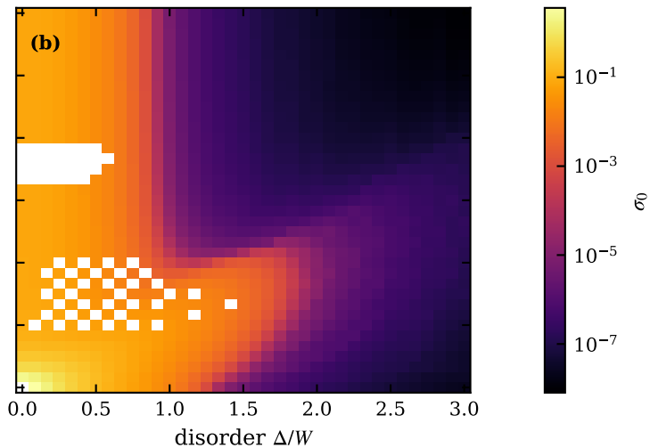
typ: \sigma(T \rightarrow 0) , n_c = 0.35
