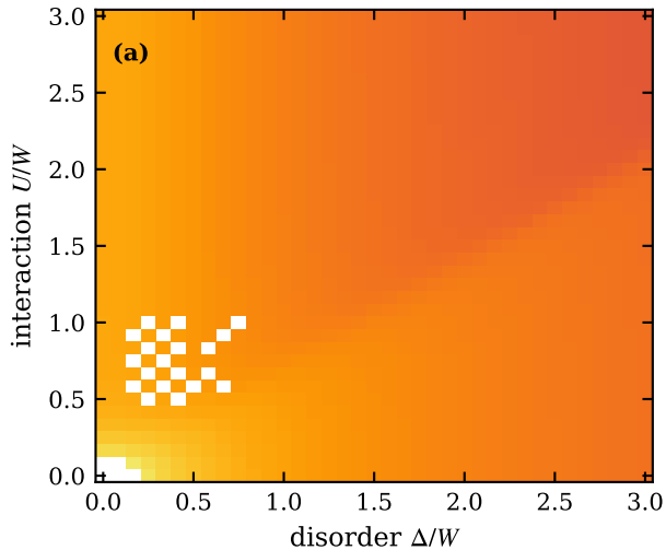
arith: \sigma(T \rightarrow 0) , n_c = 0.35
