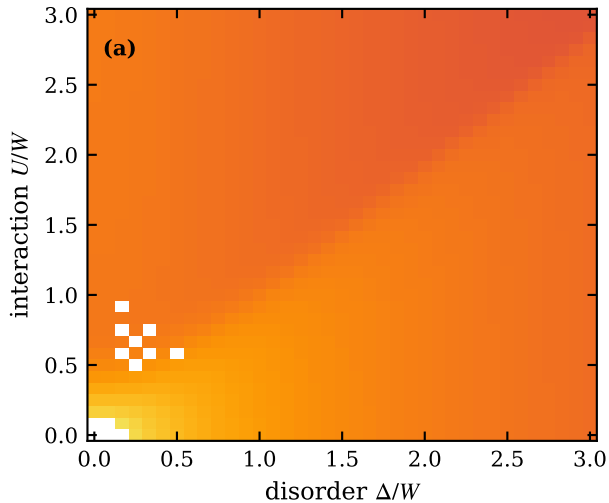
arith: \sigma(T \rightarrow 0) , n_c = 0.475
