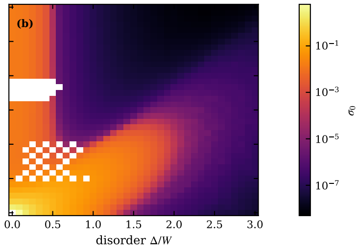
typ: \sigma(T \rightarrow 0) , n_c = 0.475
