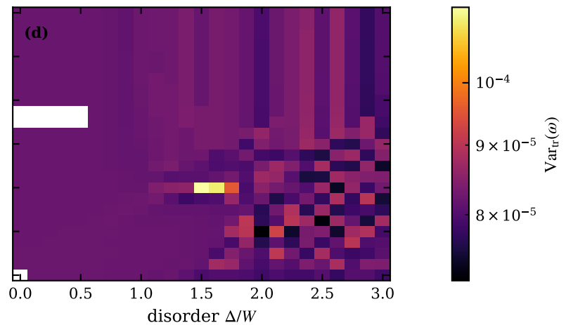
typ, n_c=0.3 , T/W=0.005
