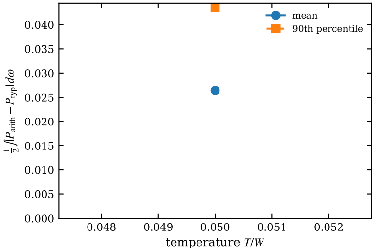
transport-shape distance near L_{12}=0 , n_c=0.35
