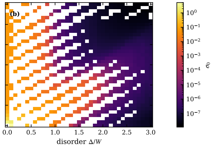
typ: \sigma(T \rightarrow 0) , n_c = 0.4 , \lambda = 0.1
