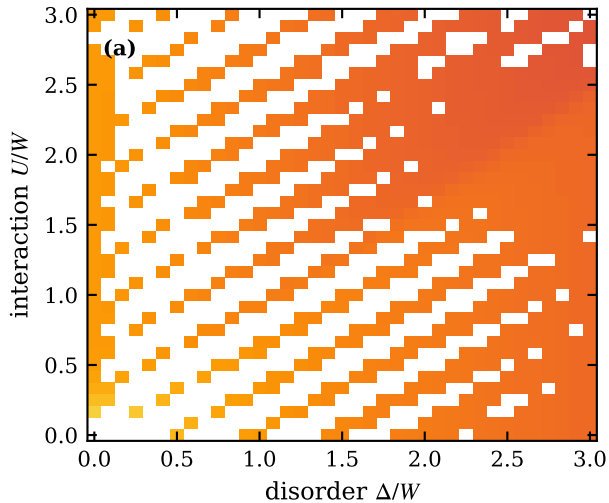
arith: \sigma(T \rightarrow 0) , n_c = 0.4 , \lambda = 0.1
