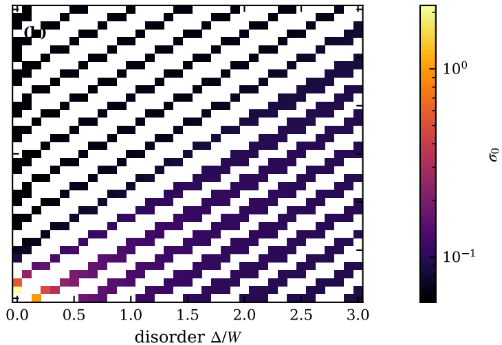
typ: \sigma(T \rightarrow 0) , n_c = 0.4 , \lambda = 1
