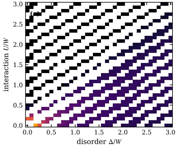
arith: \sigma(T \rightarrow 0) , n_c = 0.4 , \lambda = 1
