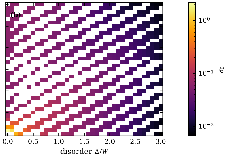
typ: \sigma(T \rightarrow 0) , n_c = 0.4 , \lambda = 1.25
