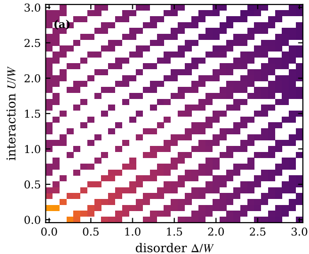
arith: \sigma(T \rightarrow 0) , n_c = 0.4 , \lambda = 1.25
