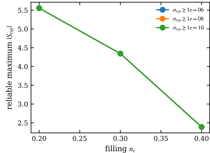
reliability test, T/W=0.02
