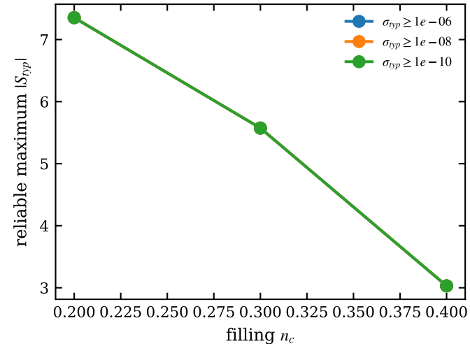
reliability test, T/W=0.05
