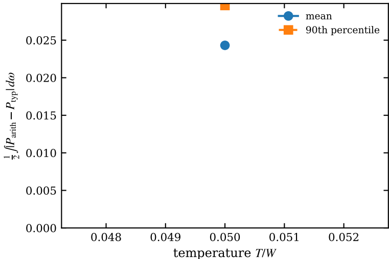
transport-shape distance near L_{12}=0 , n_c=0.325
