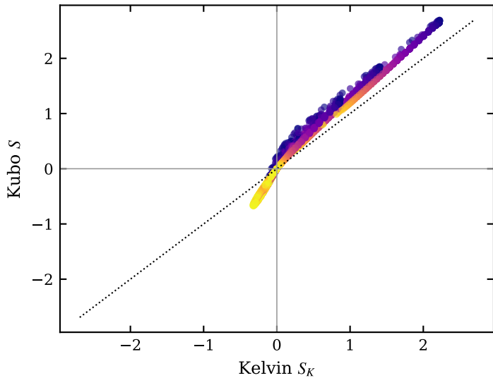
arith
