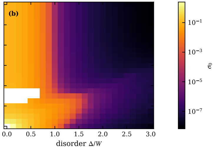
typ: \sigma(T \rightarrow 0) , n_c = 0.25
