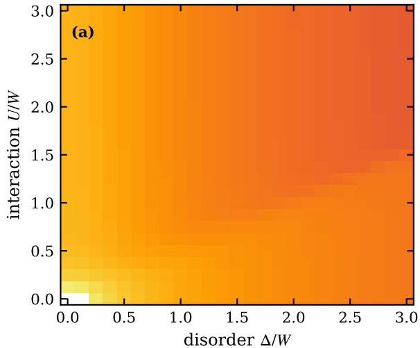
arith: \sigma(T \rightarrow 0) , n_c = 0.25
