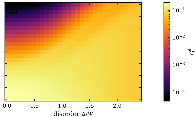
typ, n_c = 0.5 , T/W = 0.05
