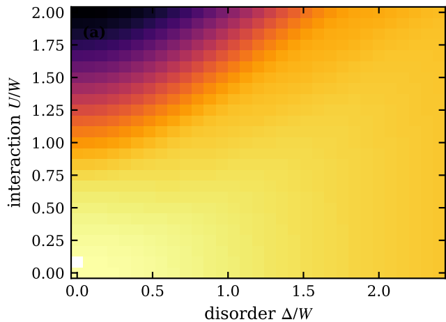
arith, n_c = 0.5 , T/W = 0.05
