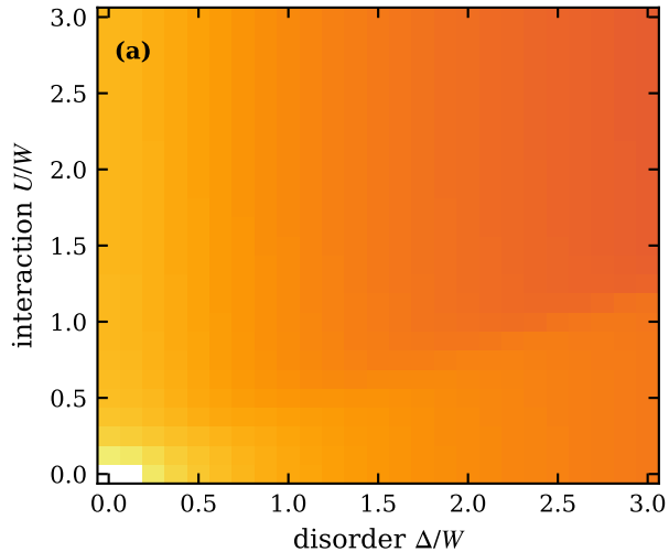
arith: \sigma(T \rightarrow 0) , n_c = 0.2
