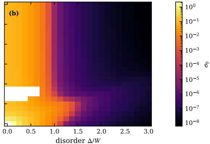
typ: \sigma(T \rightarrow 0) , n_c = 0.2
