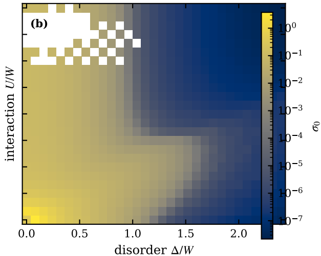
typ: \sigma(T \rightarrow 0) , n_c = 0.75
