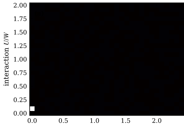
arith, n_c=0.5 , T/W=0.01
