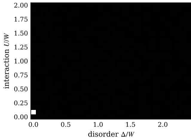
arith, n_c=0.5 , T/W=0.01
