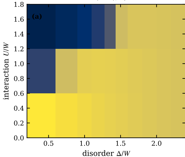
arith: \sigma(T \rightarrow 0) , n_c = 0.5
