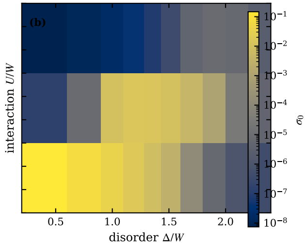
typ: \sigma(T \rightarrow 0) , n_c = 0.5
