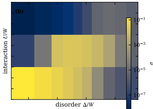
typ, n_c = 0.5 , T/W = 0.0075
