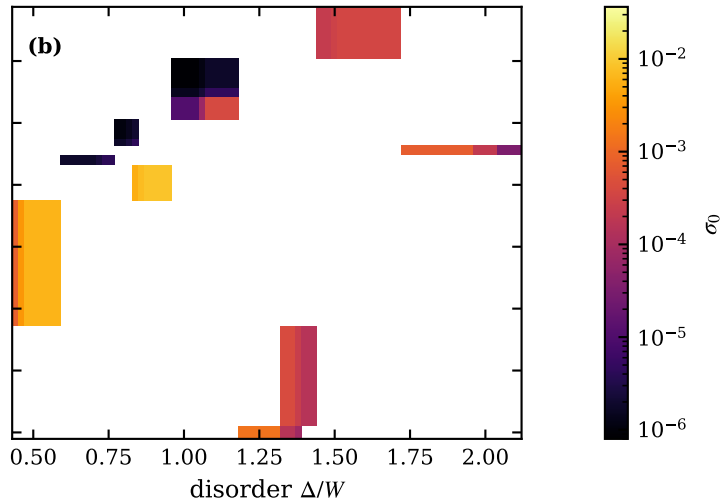
typ: \sigma(T \rightarrow 0) , n_c = 0.5
