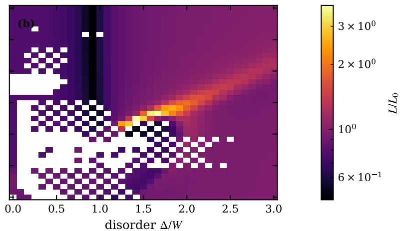
typ, n_c = 0.325 , T/W = 0.05
