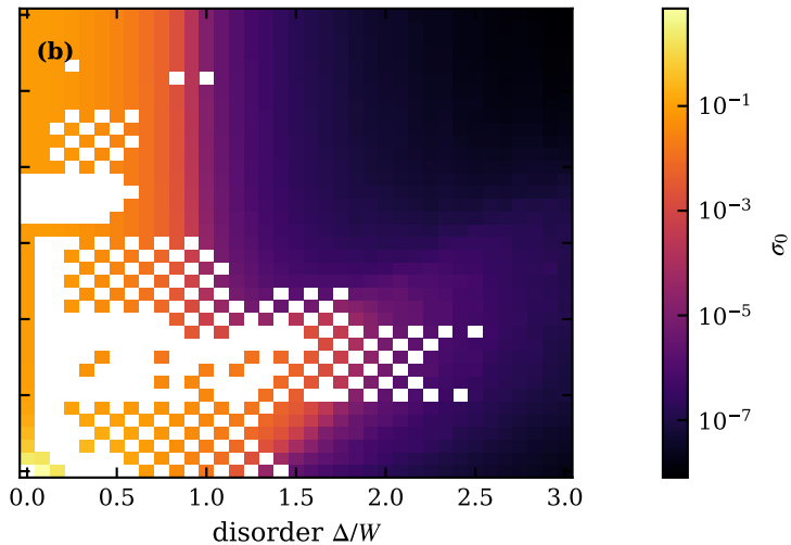
typ: \sigma(T \rightarrow 0) , n_c = 0.325
