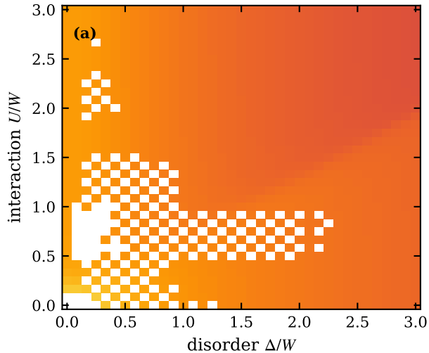
arith: \sigma(T \rightarrow 0) , n_c = 0.325
