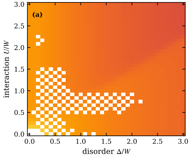
arith: \sigma(T \rightarrow 0) , n_c = 0.375
