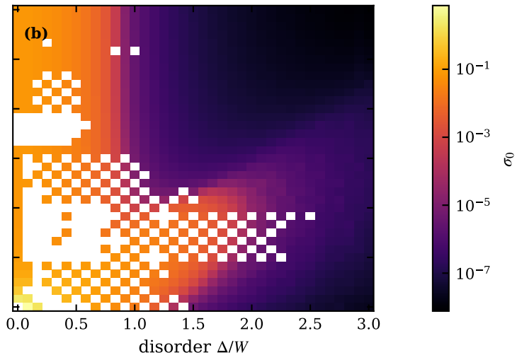
typ: \sigma(T \rightarrow 0) , n_c = 0.375
