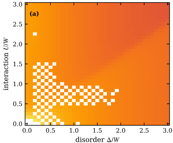
arith: \sigma(T \rightarrow 0) , n_c = 0.425
