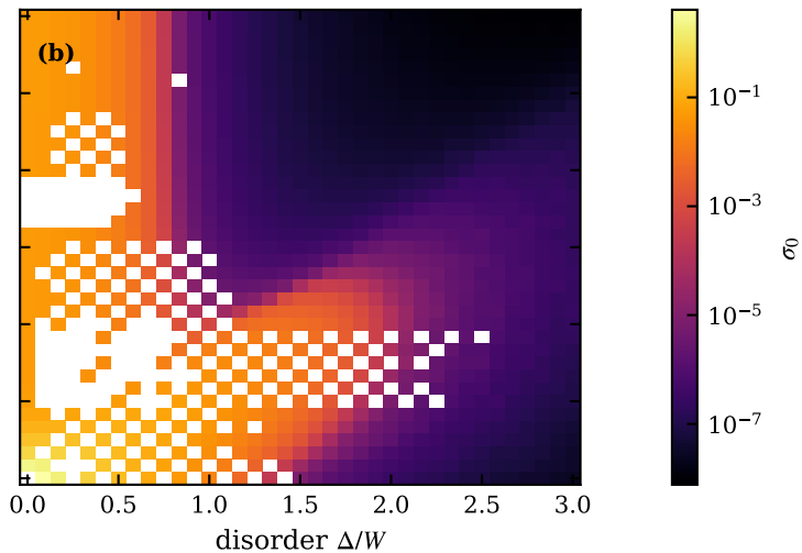
typ: \sigma(T \rightarrow 0) , n_c = 0.425
