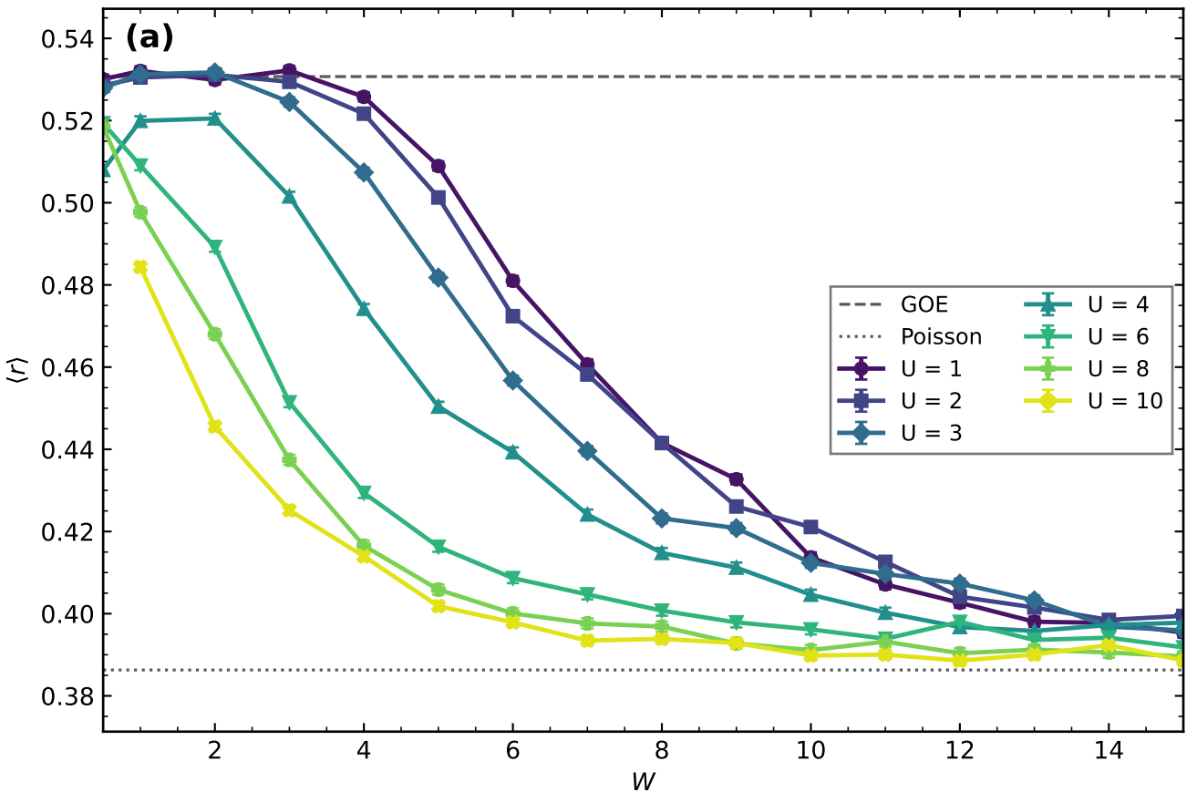
Average adjacent gap ratio \langle r \rangle
