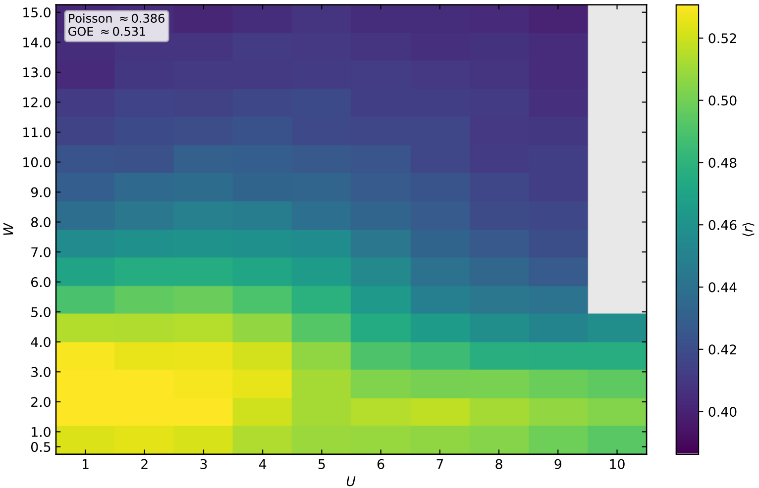
Average adjacent gap ratio \langle r \rangle
