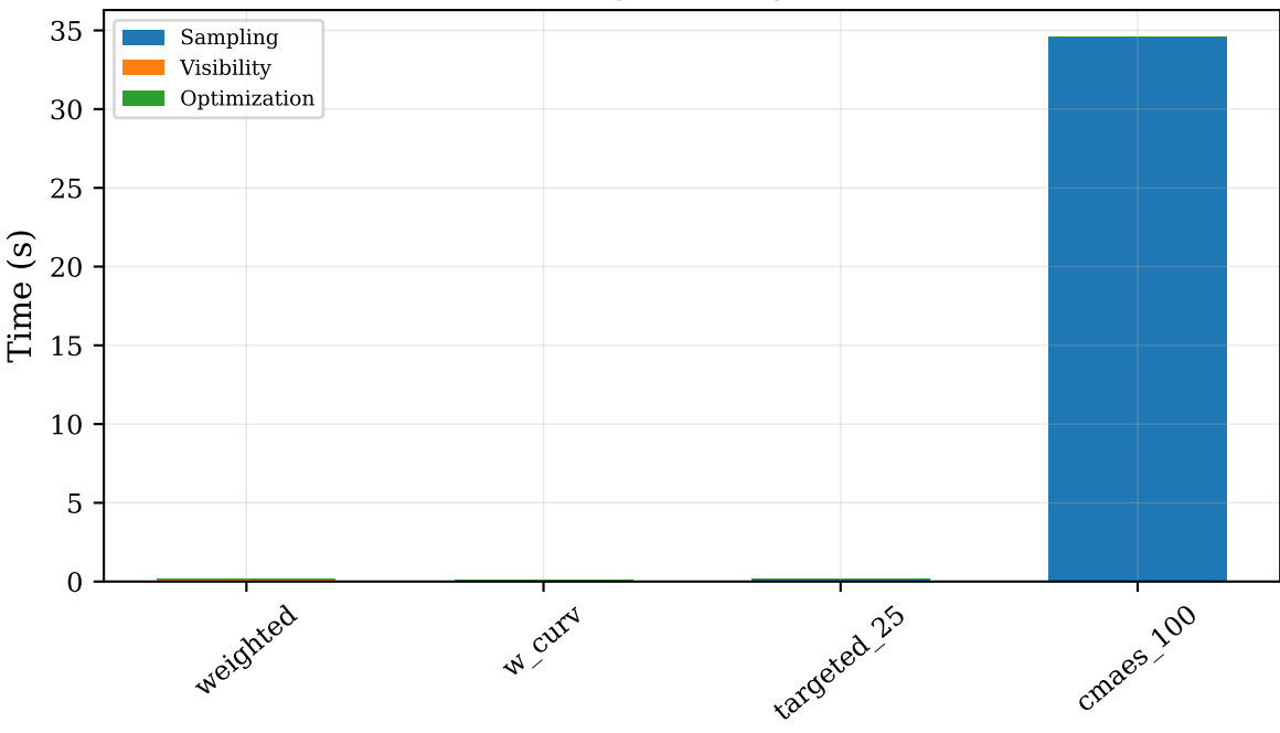
Per-Stage Timing (cat0)
