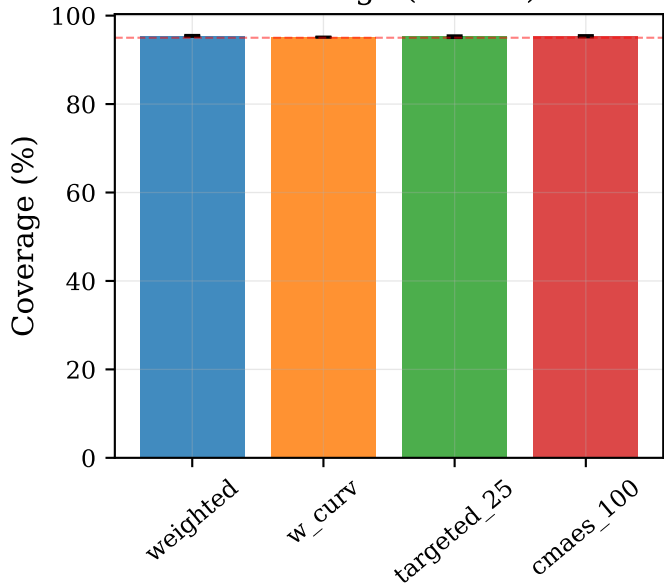
Coverage (david0)
