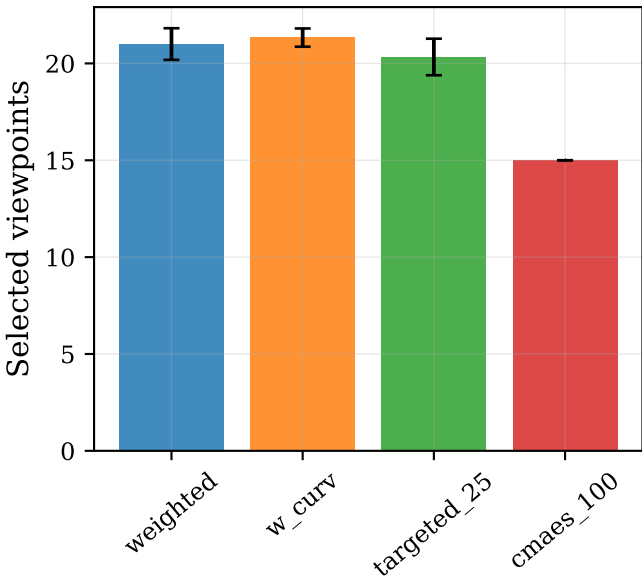
Viewpoints (david0)
