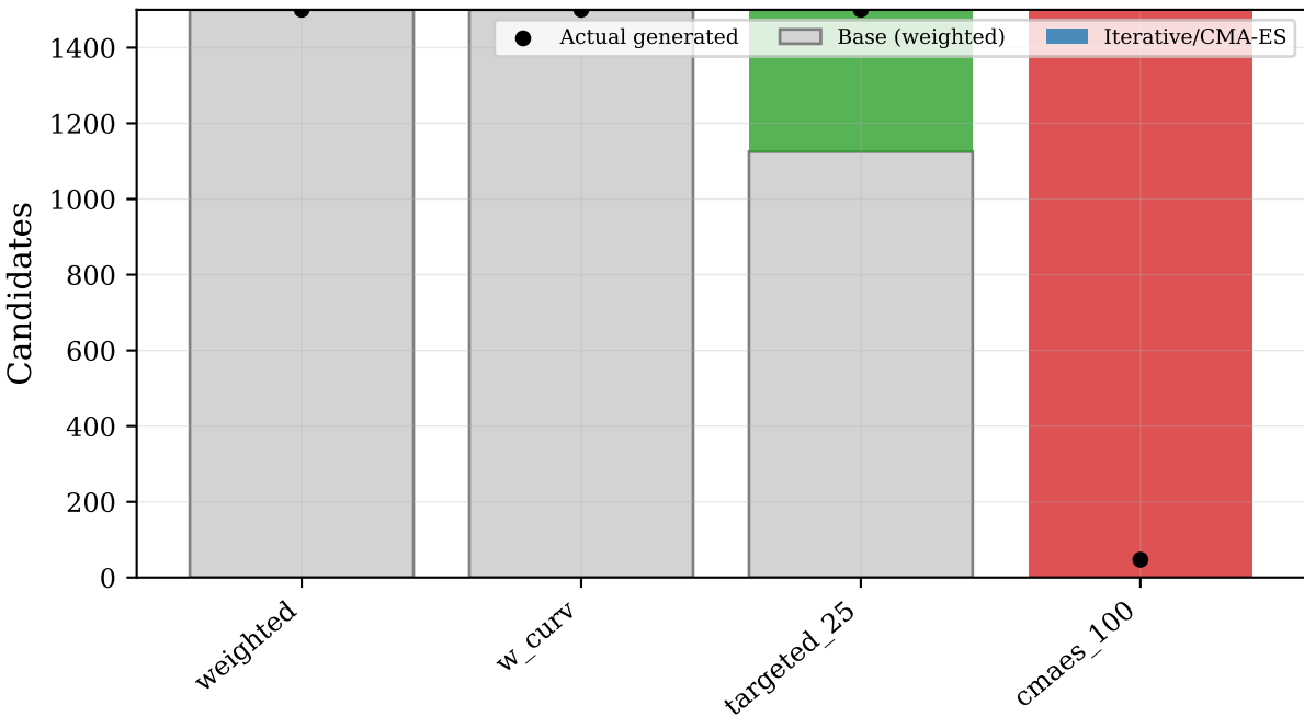
Candidate Split: Base vs Iterative (duke_of_lancaster) Base sampler for hybrid strategies: weighted
