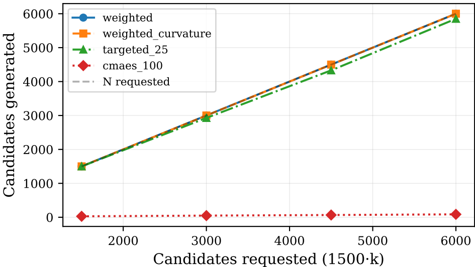
CMA-ES Early Stopping vs k-Coverage (TOSCA)
