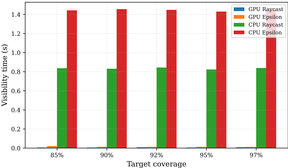
Visibility Timing: GPU vs CPU, Raycast vs Epsilon (wolf0)
