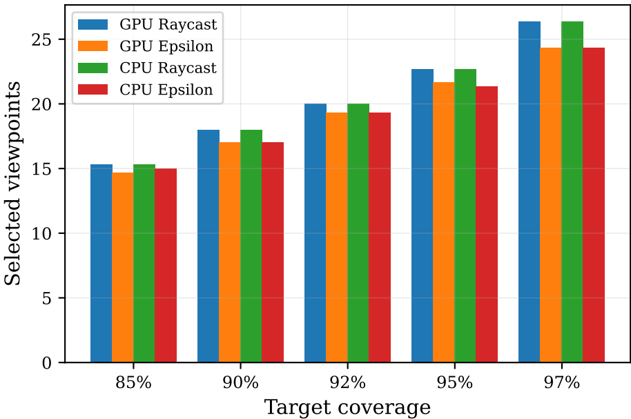
Viewpoints Selected (wolf0)
