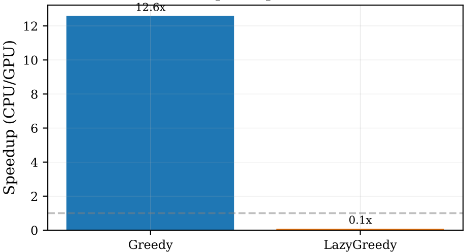
GPU Speedup (david0)
