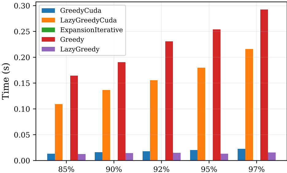
Optimization Time (david0)
