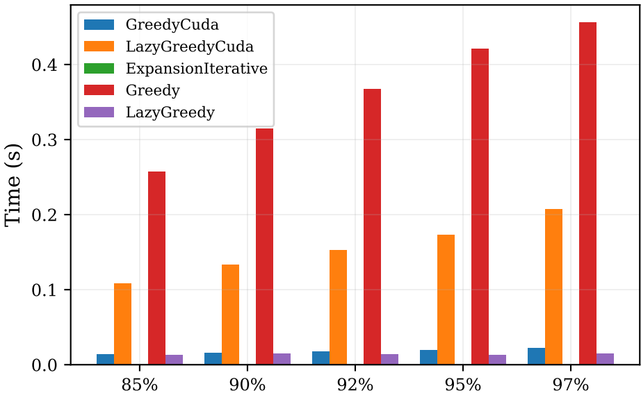
Optimization Time (wolf0)
