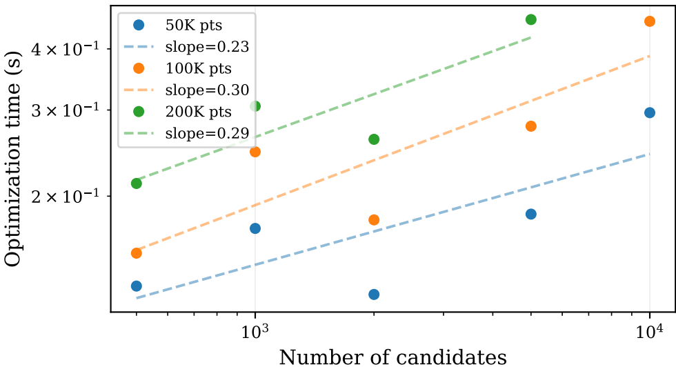
Set Cover Scaling (candidates)
