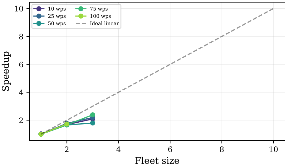
Makespan Speedup vs. Fleet Size
