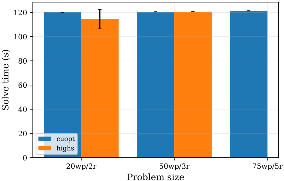
VRP Solve Time by Solver
