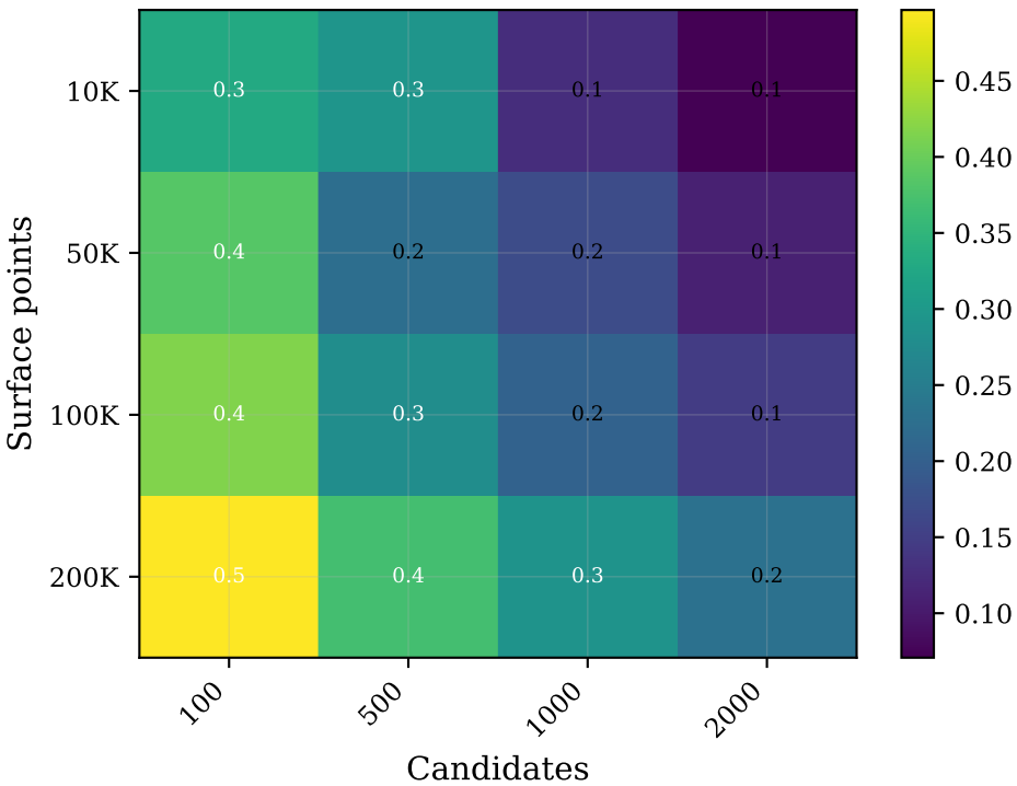
GPU Speedup (total)
