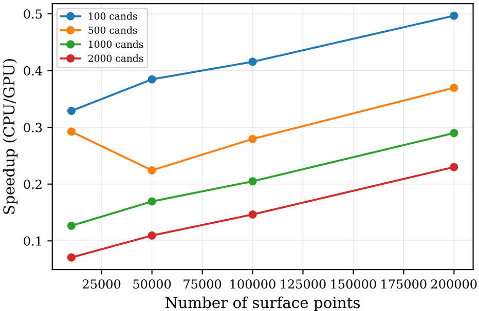
GPU Speedup vs Problem Size
