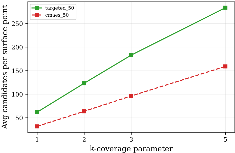
Candidate Pool Redundancy vs k (target=95%)
