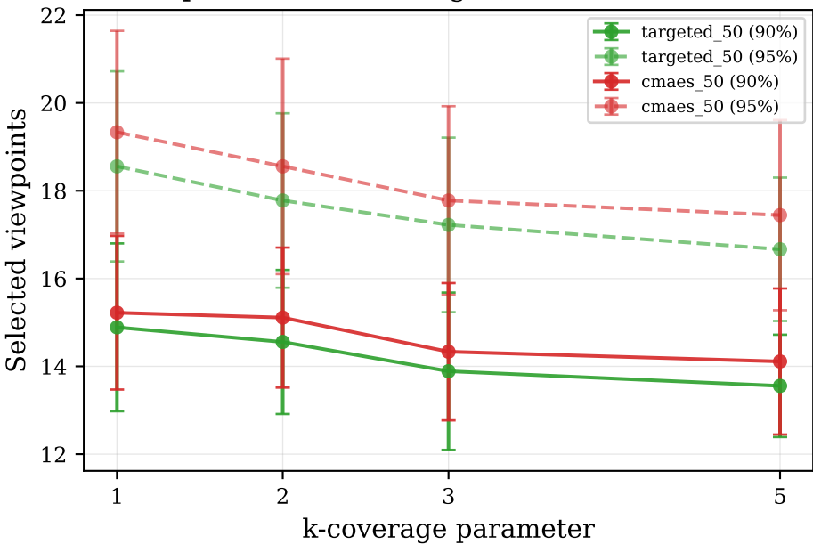
Viewpoints vs k-Coverage (N=1500·k, TOSCA)
