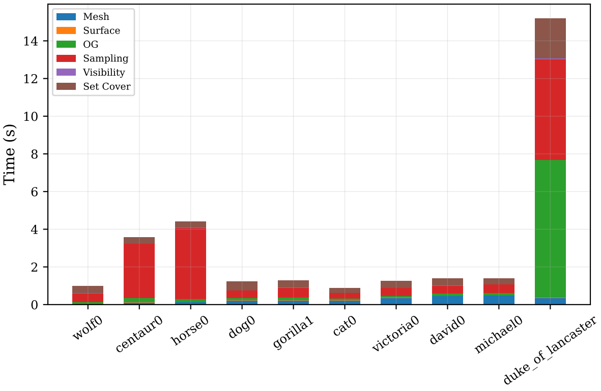
Time Breakdown by Model
