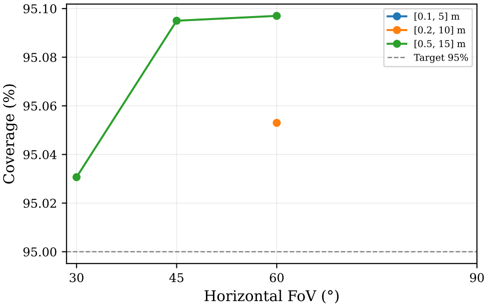
Coverage vs FoV (Duke)
